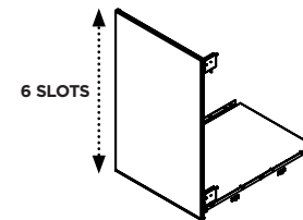
LARGE COMPARTMENT KIT ELITE ADDO-0022-A050 I.D: 25"Lx16"Wx29.5"H
