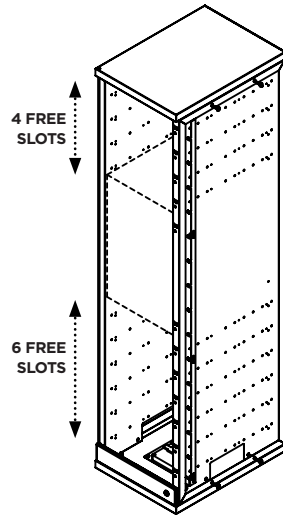
HOST SHELL KIT ELITE ADDO-0023-A070 O.A: 26"Lx19"Wx81.5"H
