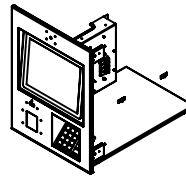
HOST COMPARTMENT KIT ELITE ADDO-0023-A020 - TOUCHSCREEN - 16 KEY KEYPAD - PORTRAIT CAMERA (OPTIONAL) - BARCODE SCANNER (OPTIONAL)
