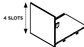
MEDIUM COMPARTMENT KIT ELITE ADDO-0022-A040 I.D: 25"Lx16"Wx19.5"H
